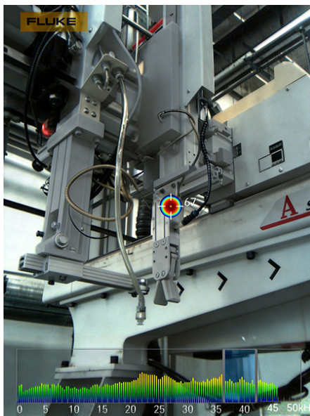
Compressed air leak detection in industrial machines
