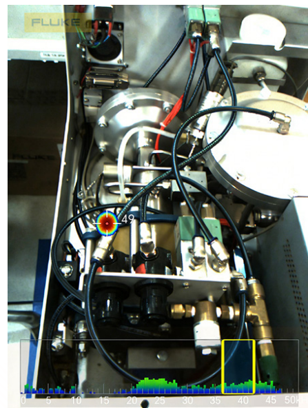
Air tightness inspection of complicated equipment pipelines
