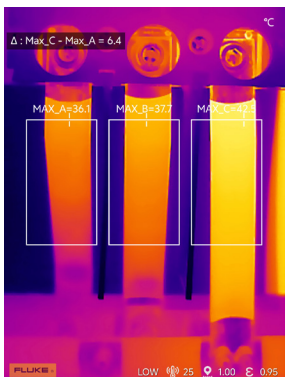
Automatic calculation of 3-phase temperature difference
