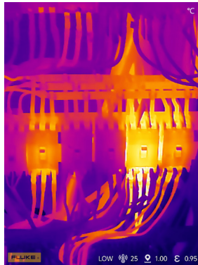
Power distribution cabinets
